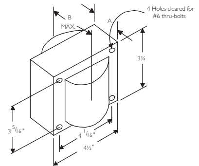
Fig. 10 (4 1/2" x 3 3/4" Reactor Core)
