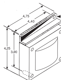
-540 Bracket Detail
