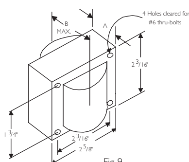
Fig 9 (2 5/8" x 2 3/16" Reactor Core)
