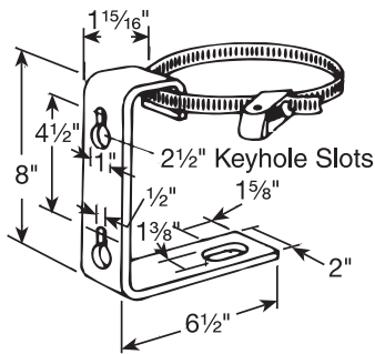
SH-I Mounting Bracket (RW4759007 and RW4777010)
