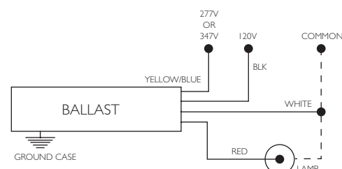
Wiring Diagram All lead lengths 12"
