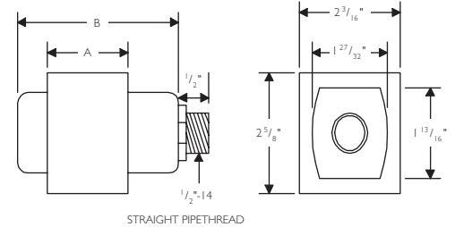
Fig 11 (J-Box Ballast)
