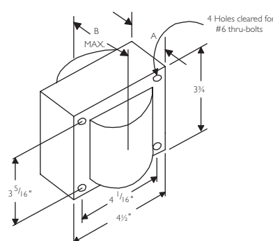
Fig. 10 (4 1/2" x 3 3/4" Reactor Core)
