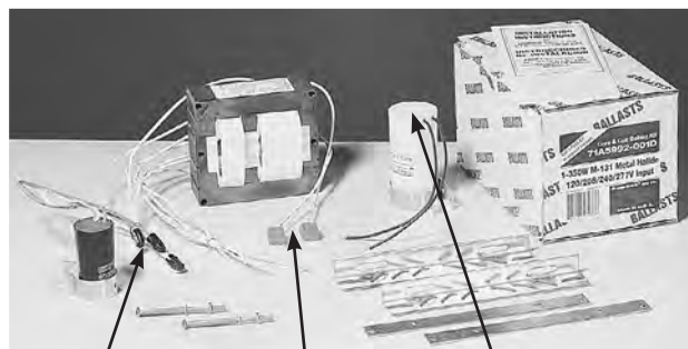
Pre-wired Ignitor
